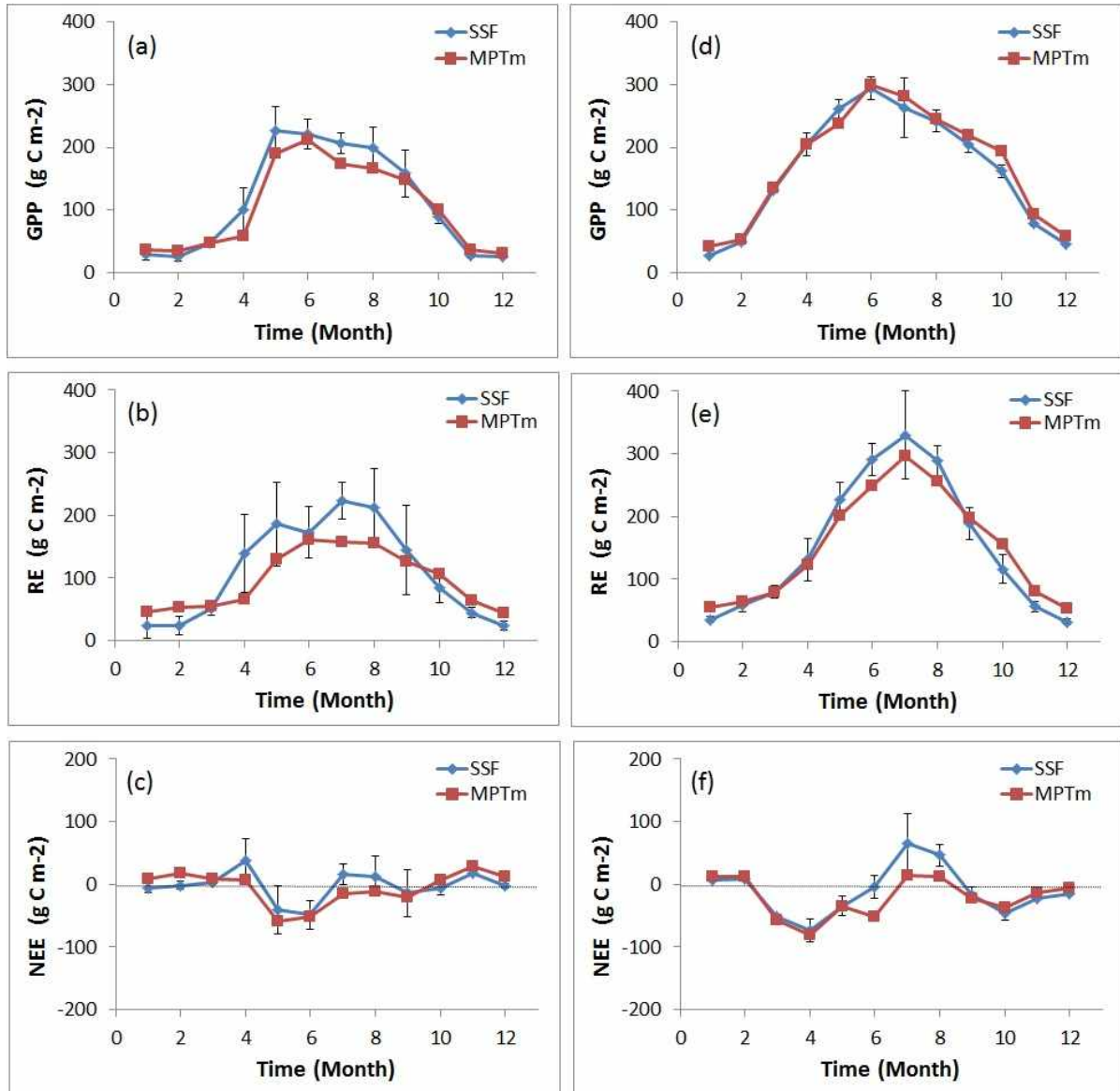
Fig. 1. Monthly gross primary production (GPP), ecosystem respiration (RE), and net ecosystem exchange (NEE) in 2009 for the GDK (a, b, c) and GCK (d, e, f). SSF indicates the site-specific filter, while MPTm indicates the modified moving point method. The error bar represents the standard deviation of the results from the three nighttime correction methods.
